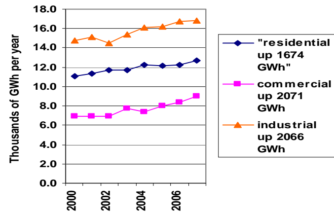
Electricity Demand March years 2000-2007
